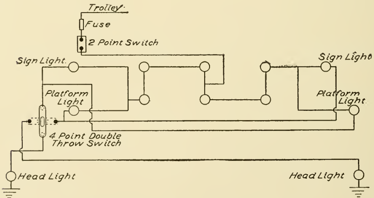
Fig. 114. Wiring Diagram for Car Lighting System
